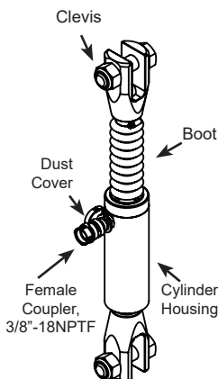
Figure 1 - HPB1006 Cylinder Components
