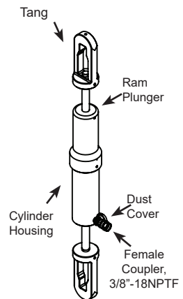
Figure 3 - HPB3006A Cylinder Components
