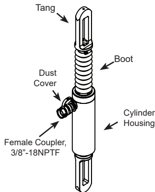
Figure 2 - HPB1006A Cylinder Components
