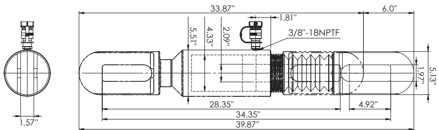
Figure 7 - HPB6006A Specifications
