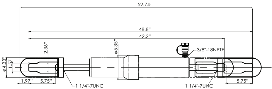
Figure 6 - HPB3006A Specifications
