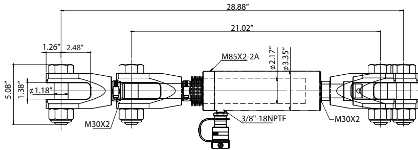
Figure 4- HPB1006 Specifications
