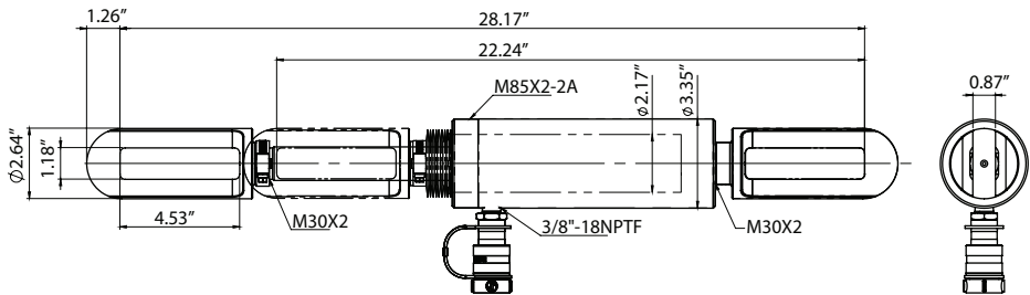
Figure 5- HPB1006A Specifications
